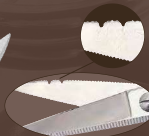
Lame esterne zigriate con spellafili un filo microdentato Ridged back edge of the blade, with 1 micro-serrated blade and wire cutting notches
